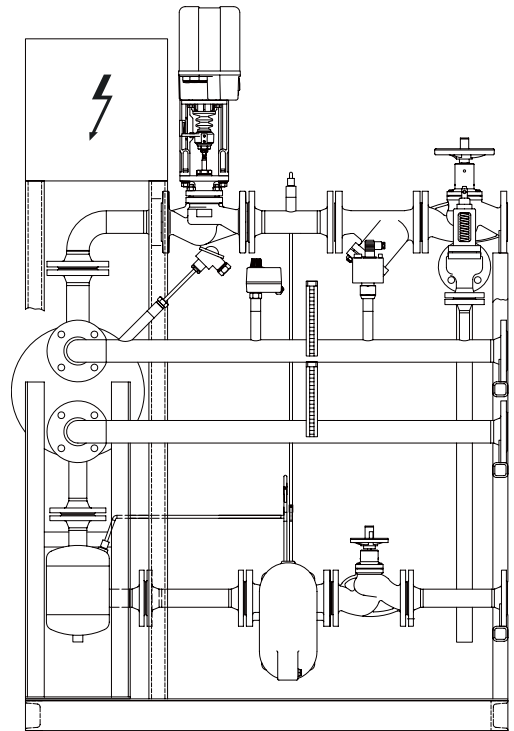
GESTRA Heat exchanger unit type PWT-XPS
