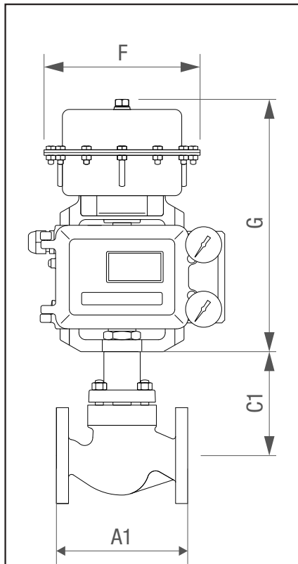
Pneumatic Actuators
