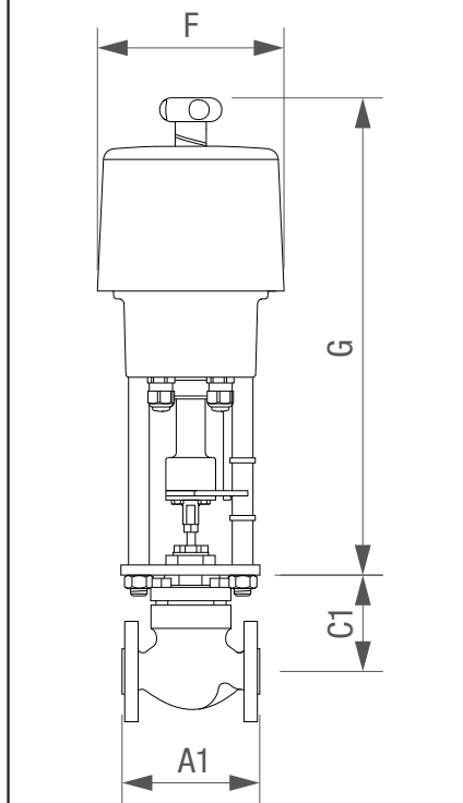
Electric Actuators
